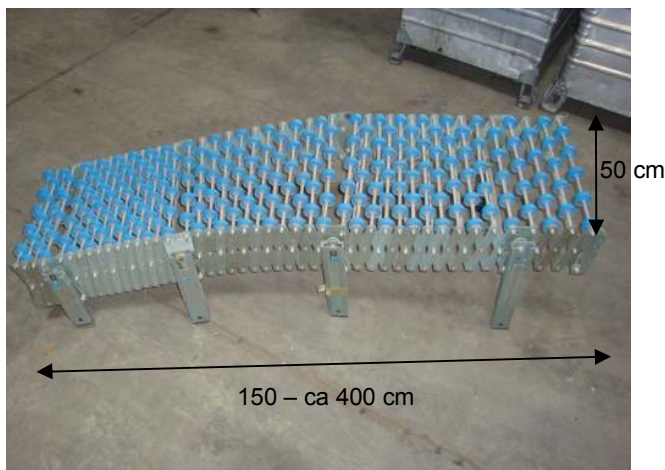
Roller conveyor 02005
